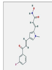
Chemical structure of MC1568
