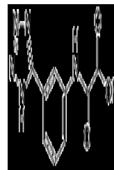
Chemical structure of Acitazanolast (WP-...)
