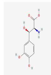
Chemical Structure of Droxidopa (L-DOPS)
