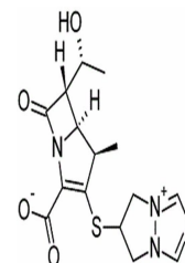
Chemical structure of Biapenem
