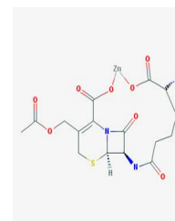
Cephalosporin C zinc salt
