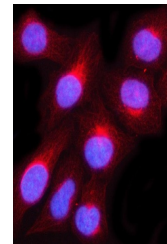
IF analysis of MUC3A/B using anti-MUC3A/...
