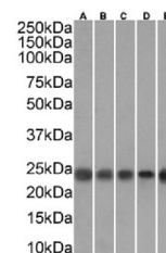
Western Blot using anti-TAGLN antibody S...
