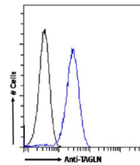
Flow cytometry using the antibody SAIC-3...
