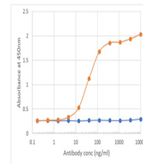
Binding curve of anti-B7-H3 antibody MJ1...
