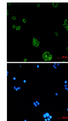
Immunocytochemistry analysis of NgR3 (gr...
