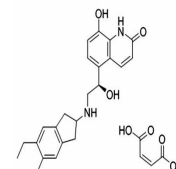
Chemical structure of Indacaterol Maleat...
