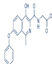
Chemical structure of Roxadustat(FG-4592...)
