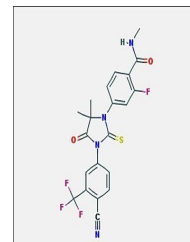
Chemical structure of Enzalutamide (MDV3...)
