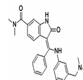
Chemical structure of BIX02189 (BIX 02189)
