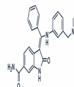
Chemical structure of BIX02188 (BIX 0218...
