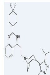
Maraviroc chemical structure
