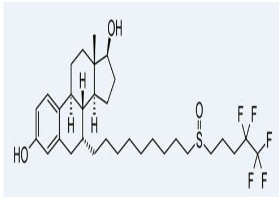
Fulvestrant chemical structure
