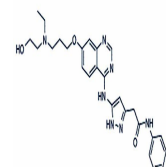
Chemical structure of Barasertib (AZD115...
