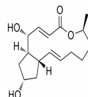
Chemical structure of Brefeldin A
