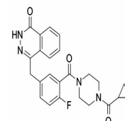
Chemical structure of AZD-2281 (Olaparib...)
