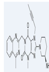
lurasidone chemical structure
