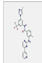
Chemical structure of Nilotinib
