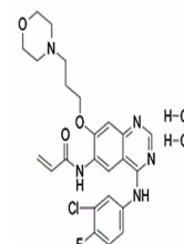
Chemical structure of Canertinib dihydro...
