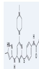
VX-680 chemical structure
