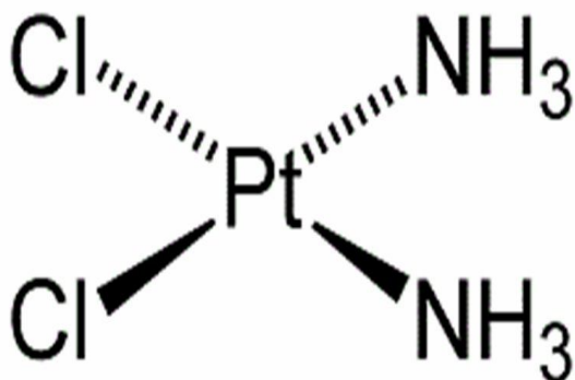
Chemical structure of Cisplatin
