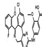
MLN8237 chemical structure
