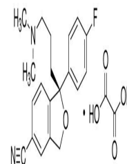
Escitalopram oxalate chemical structure
