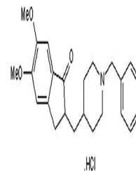
Donepezil hydrochloride chemical structu...
