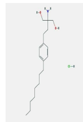
Chemical structure of Fingolimod, Hydroc...
