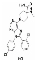
Chemical structure of CP-945598
