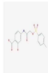
Chemical structure of S3I-201
