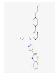
Chemical structure of Dasatinib monohydr...
