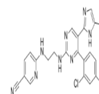
Chemical structure of CHIR-99021
