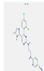
Chemical structure of CHIR-99021
