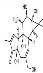
Phorbol: 4-alpha-PHR, 4-alpha-Phorbol
