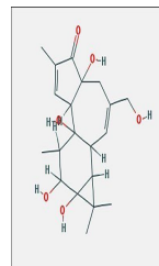
Chemical structure of Phorbol
