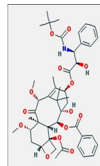
Chemical structure of Cabazitaxel
