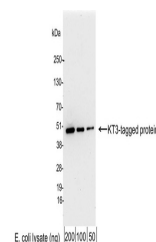
Detection of KT3-tagged protein by western blotting.
