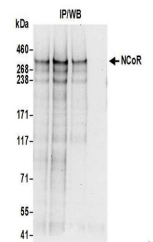
Detection of human NCoR by western blot ...
