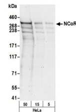
Detection of human NCoR by western blot....
