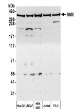
Detection of human SMG1 by western blot....
