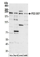
Detection of human PDZ-GEF1 by western b...
