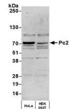
Detection of human Pc2 by western blot. ...
