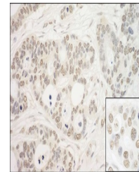
Detection of human PRP6 by immunohistochemistry.
