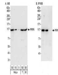
Detection of human and mouse PRP6 by western blotting.
