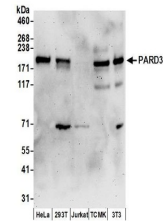
Detection of human and mouse PARD3 by we...
