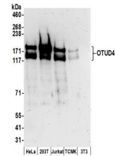
Detection of human and mouse OTUD4 by we...
