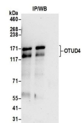
Detection of human OTUD4 by western blot...
