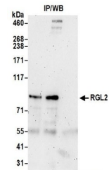
Detection of human RGL2 by western blot ...
