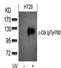
Western blot analysis of c-Cbl(phospho-T...
