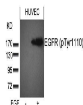
Western blot analysis of EGFR(phospho-Ty...
