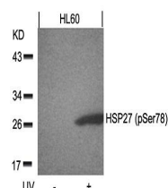
Western blot analysis of HSP27(Phospho-S...
