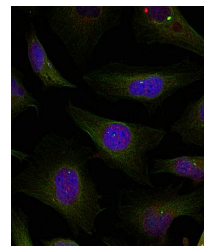
Confocal immunofluorescent analysis of HDAC4/HDAC5/HDAC9
