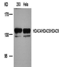
Western blot analysis of HDAC4/HDAC5/HDAC9
