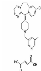
Chemical structure of Rupatadine
