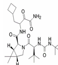
Chemical structure of Boceprevir(EBP 520...
