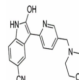
Chemical structure of AZD1080
